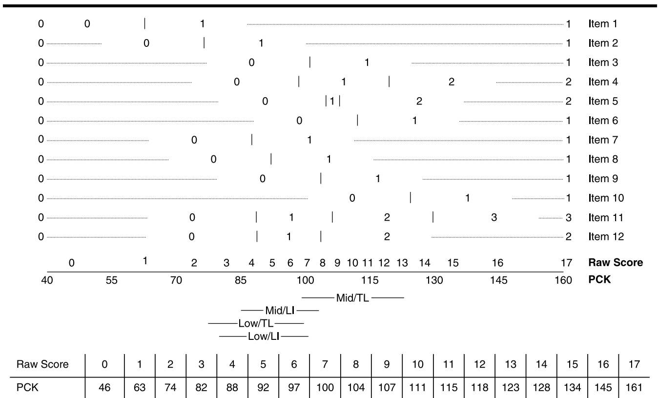
Figure 1. Trait map depicting print-concept knowledge estimates.
