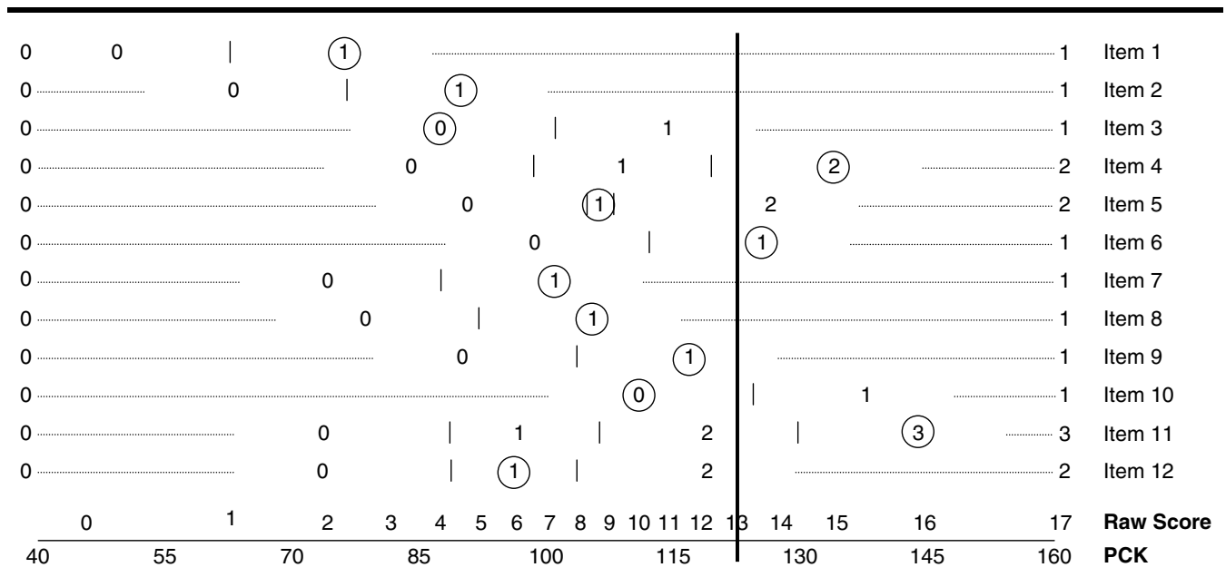
Figure 2. Example of use of a print-concept knowledge trait map.
